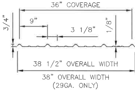
Tuff-Rib PANEL PROFILE
